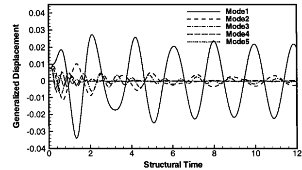
Fig. 14 Time history of the generalized coordinates for the AGARD 445.6 wing for M_\infty = 1.072 and V_f = 0.46 .
