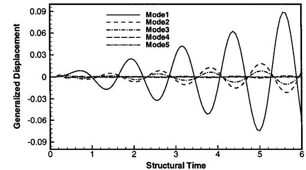
Fig. 13 Time history of the generalized coordinates for the AGARD 445.6 wing for M_\infty = 1.141 and V_f = 0.70 .
